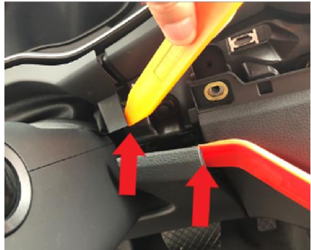
10. Pry the instrument cluster lower trim and the driver knee board panel slightly to remove the center dash trim. It is not necessary to remove them completely, but to create a bit of space to take out the center dash trim with climate control.
