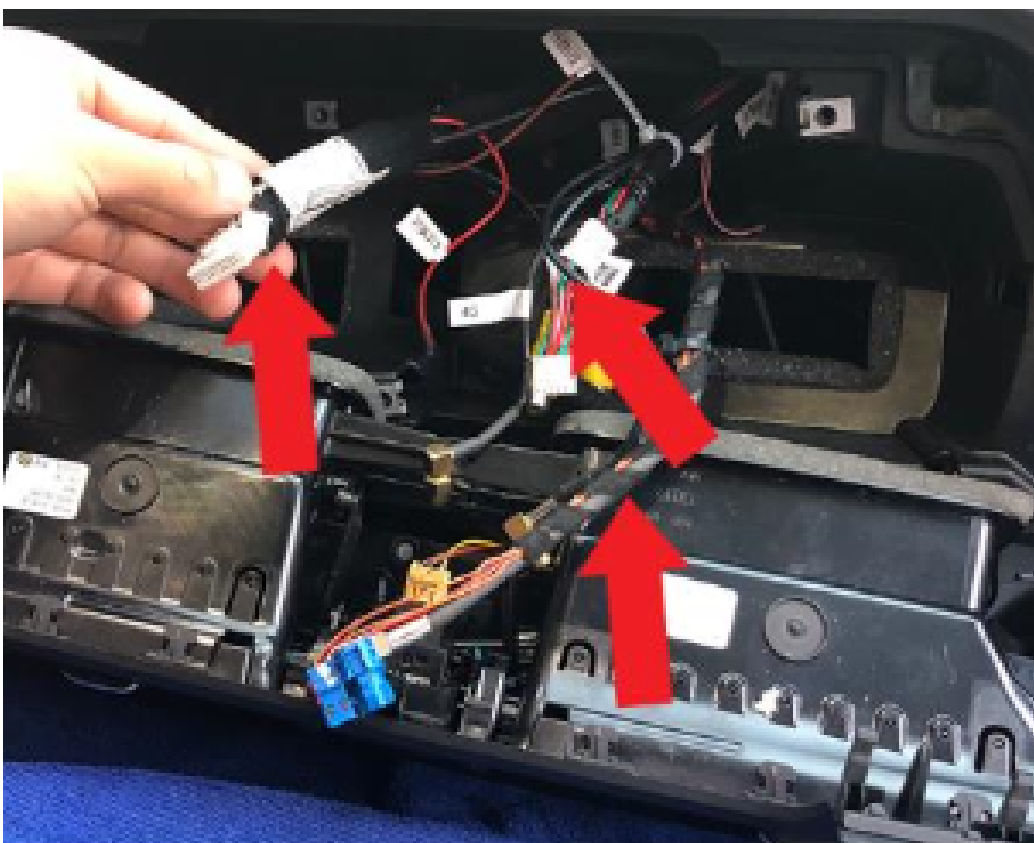
17. Route the cable into the screen opening by passing it behind the air ducts from the glove box.
