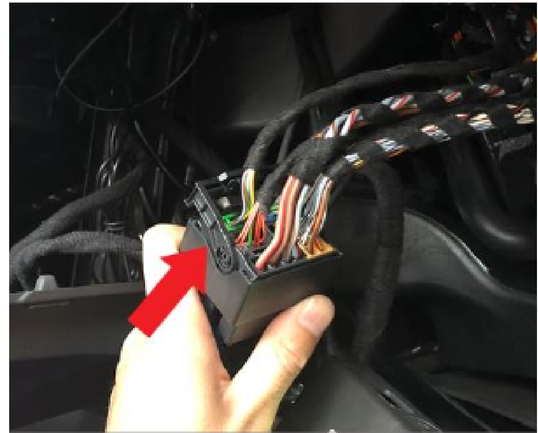
16. Install the provided main harness by routing the white main connector to the LCD screen area.
