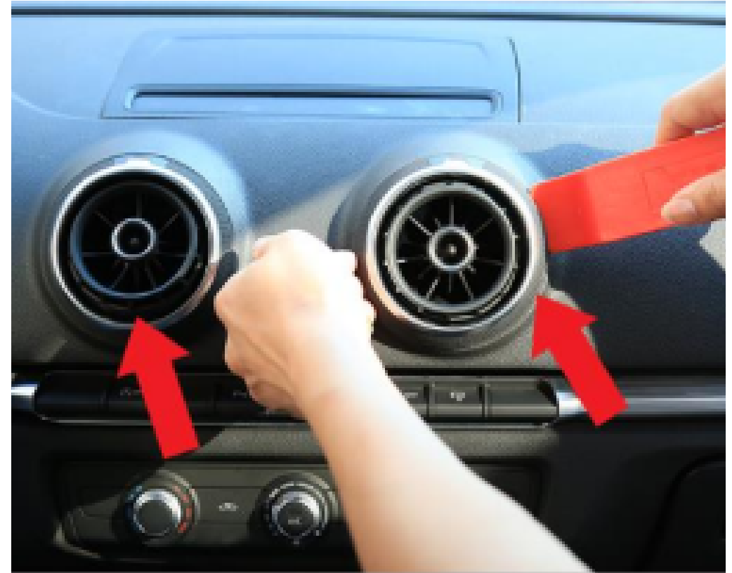
2. Using a prying tool, remove the center air vents.
